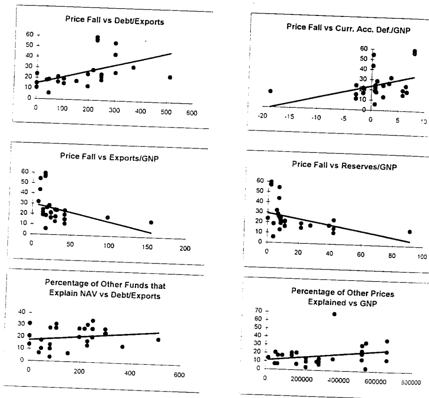
Figure 8.3. Fundamentals-contagion relationships.
